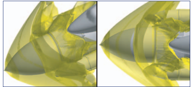
Figure 5-2. Mach number isosurfaces at Mach number = 2.46.
