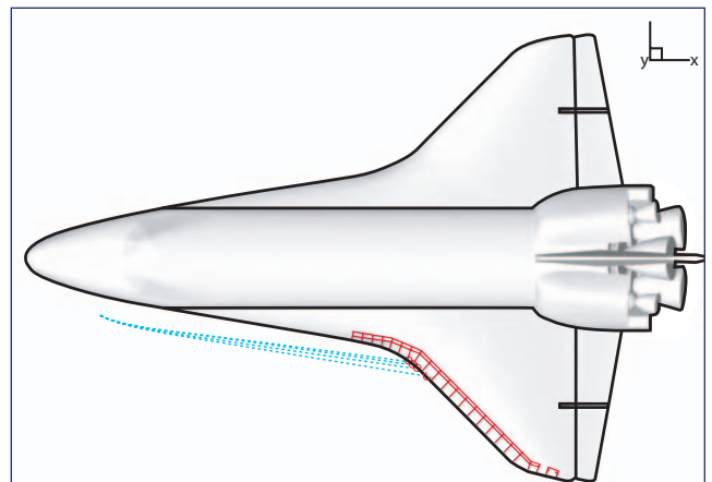
Figure 7-14. Top view of optimized foam debris trajectories for index intervals 7-13, 7-14, 7-15, 7-16, 8-13, 8-14, 8-15, and 8-16, projected to Shuttle impact and showing outboard direction of trajectory at impact. Graphic courtesy of Phil Stuart – JSC/EG3.
