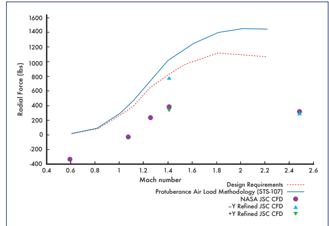
Figure 14-4. -Y Bipod ramp radial force vs. Mach number.
