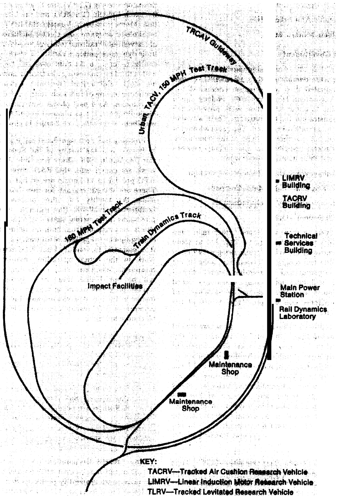
FIGURE 72 DOT Test Track, Pueblo, Colorado
