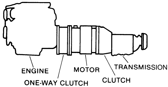
Figure 4.4 Power Train of Daihatsu 1.5-ton Hybrid Truck
