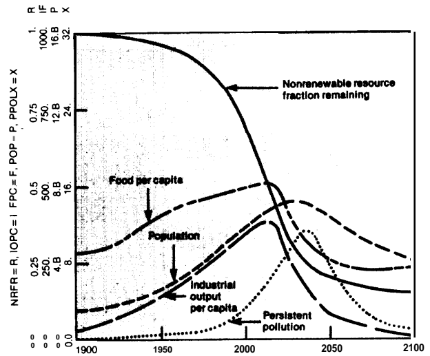
Run 7-6A: World 3 reference run.
