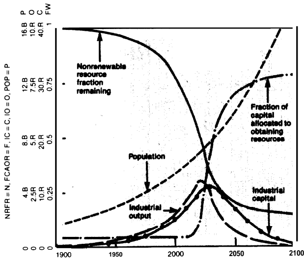
Run 5-1: standard run for the nonrenewable resource sector.
