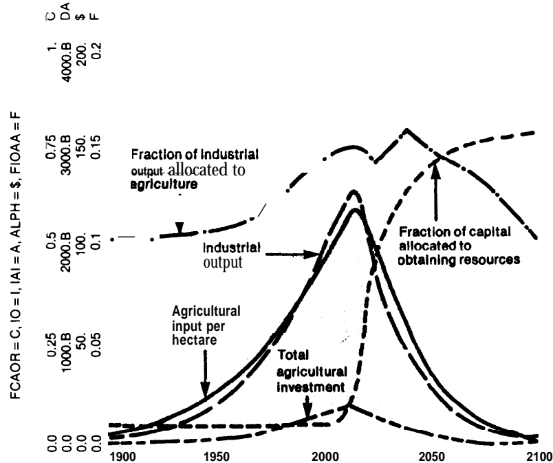
Figure B-2.—Output From Standard Simulation of World 3
