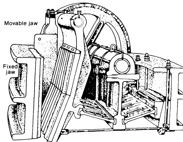
Figure 6-15.—Jaw Crusher
