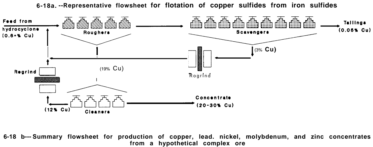
Figure 6-18.-Flowsheets for Copper Flotation
