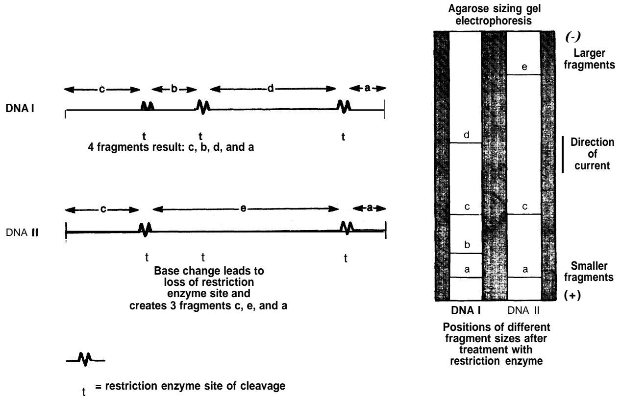
Figure 7.—Production of Restriction Fragment Length Polymorphisms Using Restriction Enzymes and Separation of Different DNA Fragment Sizes by Agarose Gel Electrophoresis
