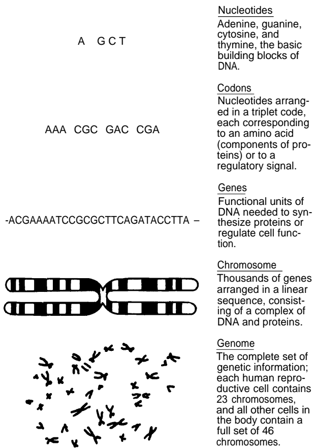
Figure 1.—Organizational Hierarchy of DNA, the Carrier of Genetic Information in Human Cells
