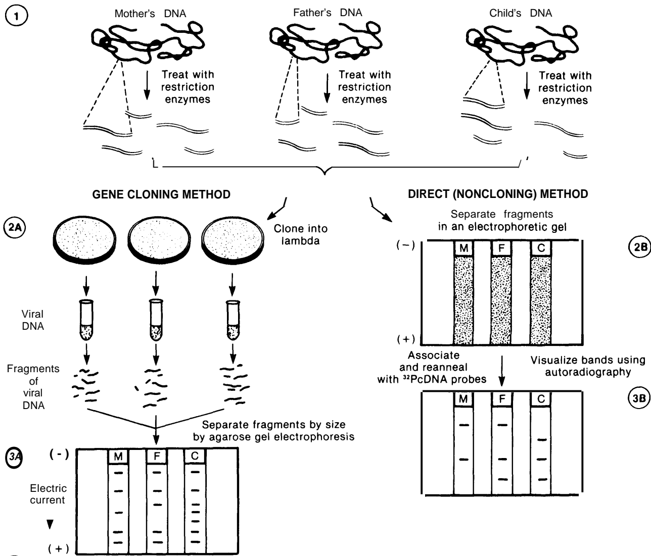
Figure 8.—Restriction Fragment Length Polymorphism
