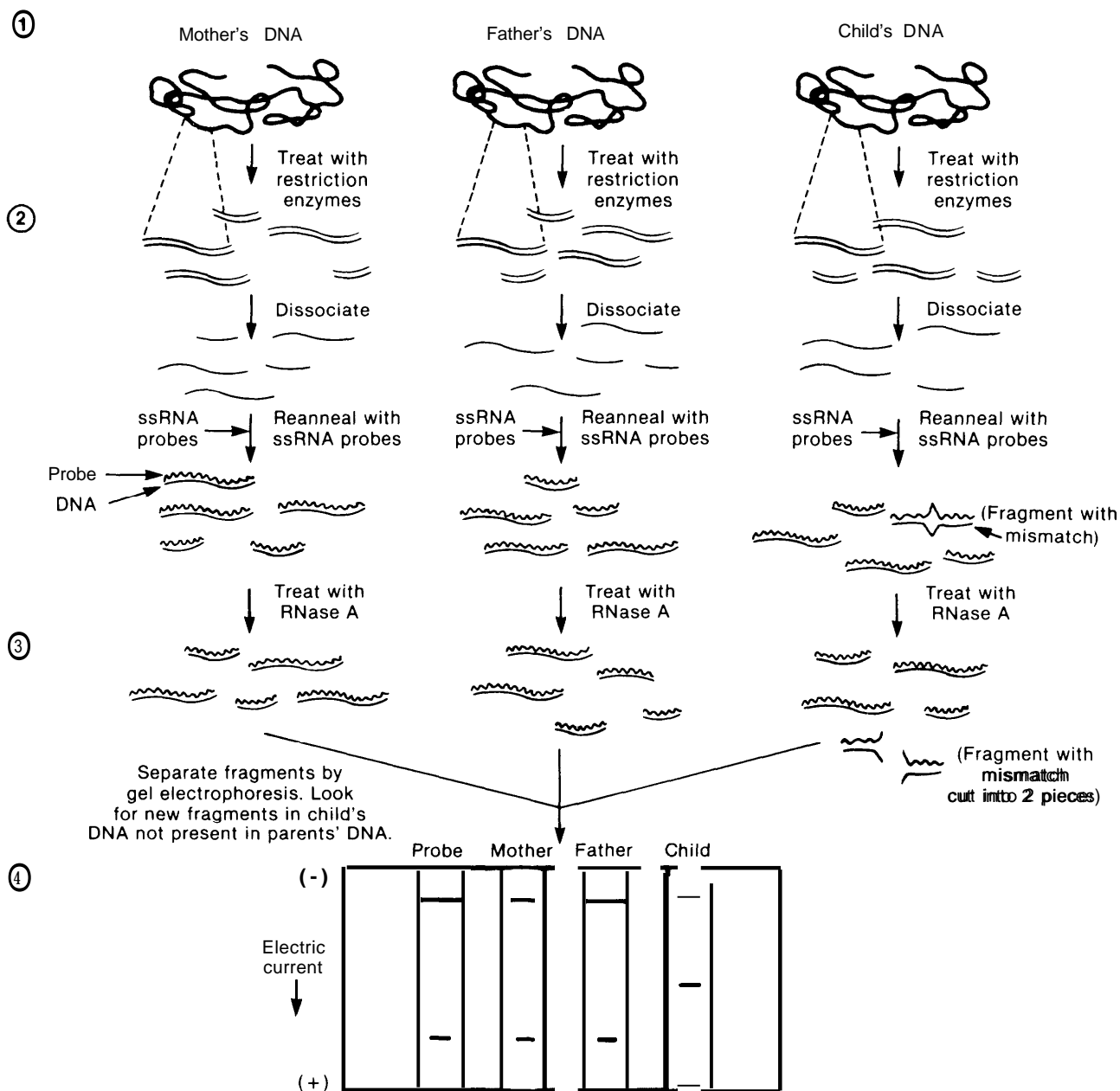
Figure 11.—Ribonuclease Cleavage of Mismatches in RNA/DNA Heteroduplexes
