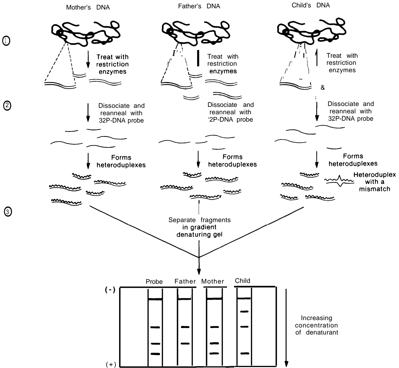
Figure 9.—One-Dimensional Denaturing Gradient Gel Electrophoresis
