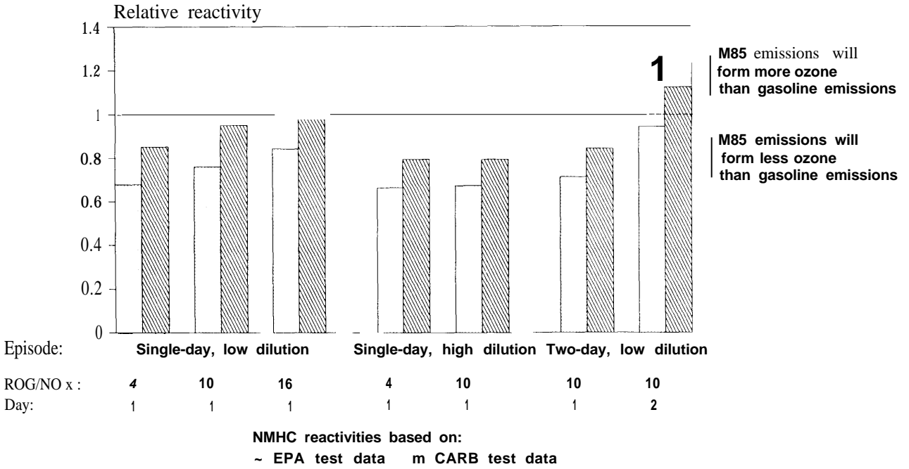
Figure 3-1—"Relative Reactivity" (Ozone-Forming Capability) of Emissions From M85-Fueled Vehicles v. Gasoline-Fueled Vehicles
