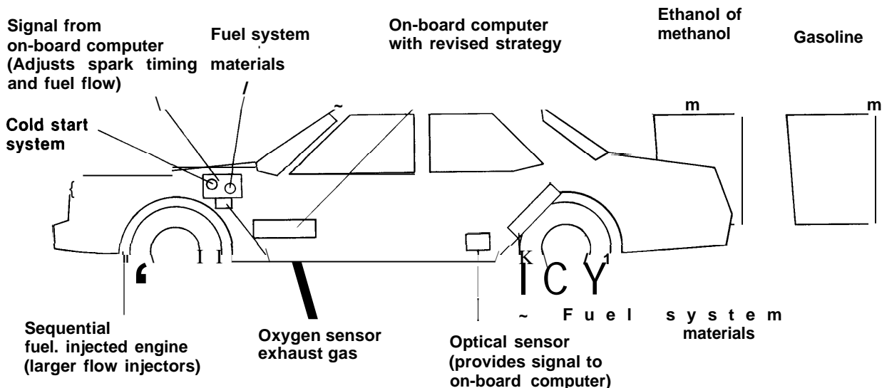
Figure 4—Technical Difference Between Flexible-Fuel and Conventional Automobiles
