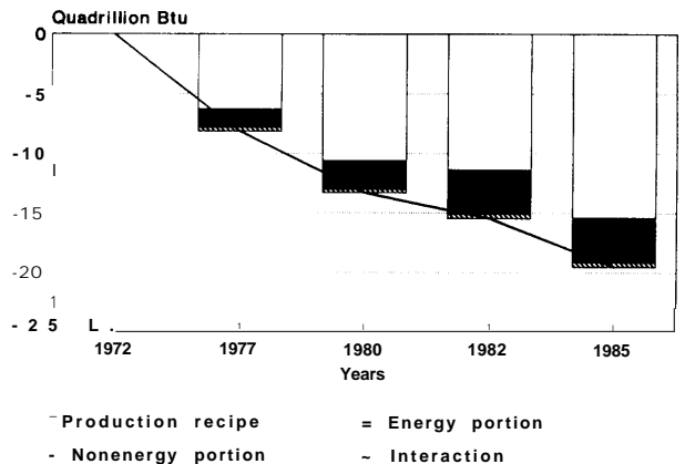
Figure 14—Changes in U.S. Energy Use Due to Changes in Production Recipe, 1972-85
