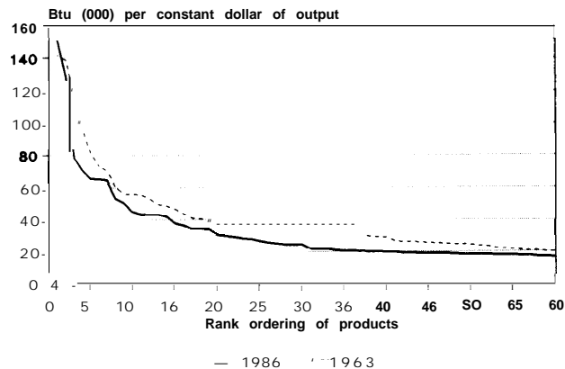
Figure 15—Ranking of Primary Energy Intensity of Selected Products
