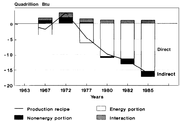
Figure 13—Changes in U.S. Energy Use Due to Changes in Production Recipe, 1963-85
