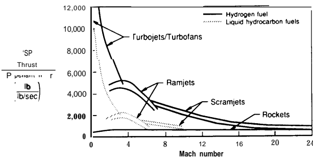
Figure 5-5—Engine I_{sp}
